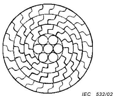
Figure 1b – Three-layer conductor made of formed wires type AxF/Sxy
