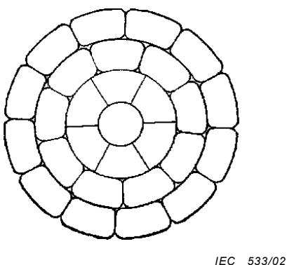
Figure 2 – Two-layer conductor made of formed wires type AxF/AyF
